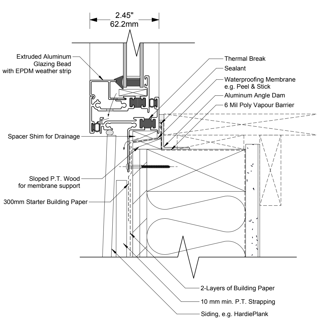
1 Casement Sill Detail Scale: 1:2
